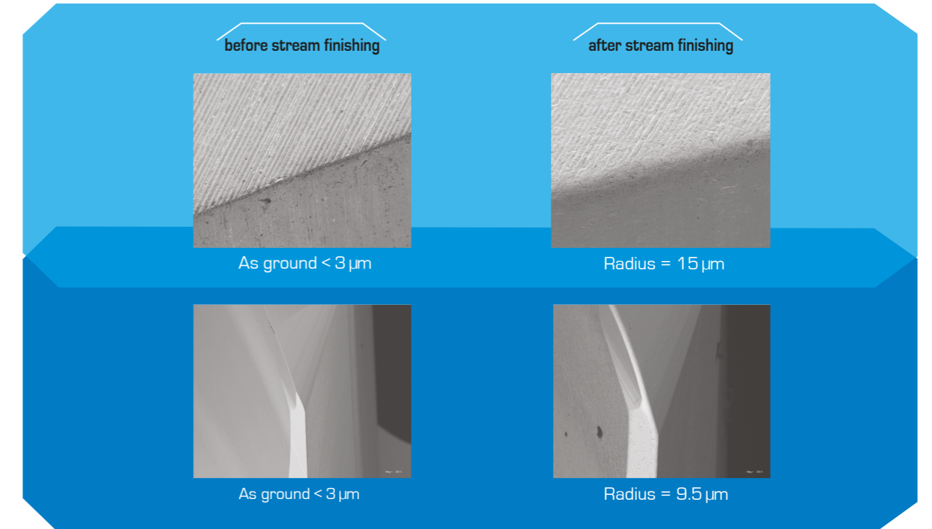
Depending on the required edge rounding, different media are applied.
